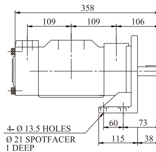
Foot Type (腳座型)
